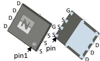
DFN5*6
