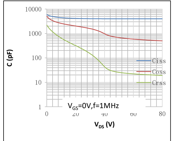
Fig.2 Capacitance Characteristics
